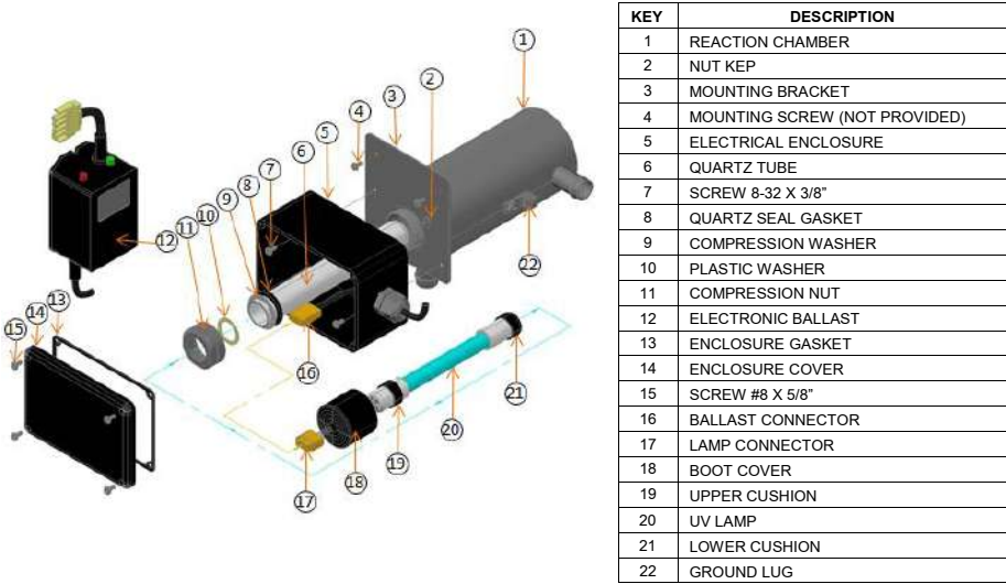
Figure 1: Exploded View
